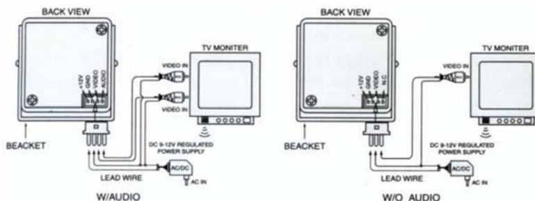
LEAD WIRE CONNECTION
